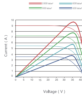
Current-Voltage & Power-Voltage Curves (315W)
